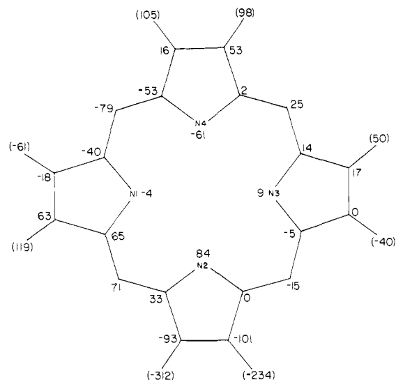
Figure 6. Displacements (in Å \times 10^3 ) of atoms from the least-squares plane of the 24-atom porphyrin skeleton. The estimated standard deviations are 0.004 Å for nitrogen atoms and 0.004–0.005 Å for carbon atoms. Displacements in parentheses were not included in the calculation of the least-squares plane.
