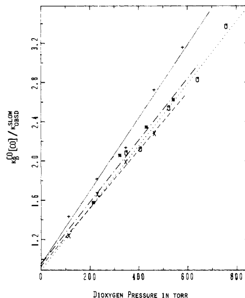
Figure 11. Plots of K_{\text{B}}^{\text{CO}}[\text{CO}]/k_{\text{obsd}}^{\text{slow}} vs. dioxygen partial pressure over toluene (0.45 M DCIm) at 20 \text{ }^\circ\text{C} : (+) [\text{CO}] = 1.75 \text{ mM}, 175 \text{ torr} , k_{\text{B}}^{\text{CO}}[\text{CO}] = 19.5 \text{ s}^{-1} , slope = 3.72 \times 10^{-3} \text{ torr}^{-1} ; (X) [\text{CO}] = 1.76 \text{ mM}, 176 \text{ torr} , k_{\text{B}}^{\text{CO}}[\text{CO}] = 18.2 \text{ s}^{-1} , slope = 2.95 \times 10^{-3} \text{ torr}^{-1} ; (O) [\text{CO}] = 1.17 \text{ mM}, 117 \text{ torr} , k_{\text{B}}^{\text{CO}}[\text{CO}] = 12.5 \text{ s}^{-1} , slope = 3.16 \times 10^{-3} \text{ torr}^{-1} ; (*) [\text{CO}] = 1.09 \text{ mM}, 109 \text{ torr} , k_{\text{B}}^{\text{CO}}[\text{CO}] = 11.0 \text{ s}^{-1} , slope = 3.15 \times 10^{-3} \text{ torr}^{-1} .
