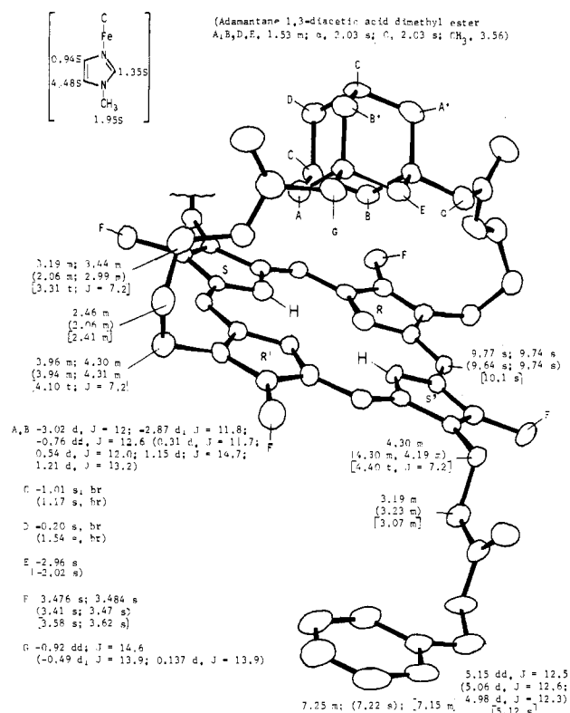
Figure 7. Nuclear magnetic resonance assignments of adamantane-porphyrin-6,6-cyclophane ( 5P ), adamantane-heme-6,6-cyclophane-1-MeIm-CO complex (MeIm-5-CO) (in parentheses), and the precursor porphyrin (strap replaced with two (CH 2 ) 3 NH 2 groups) in chloroform (in brackets). Insets give free adamantane and bound imidazole assignments. Chemical shifts are in ppm downfield from Me 4 Si.
