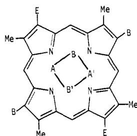
Figure 8. Symmetry relationships of the methylene groups labeled A, A', B, and B' in Figure 7 as the adamantane adopts the left (unprimed) (CH 2 ) s down conformation or the right (primed) (CH 2 ) s down conformation. The side chains are carbobenzyoxyethyl (E) and cyclophane bridge (B).
