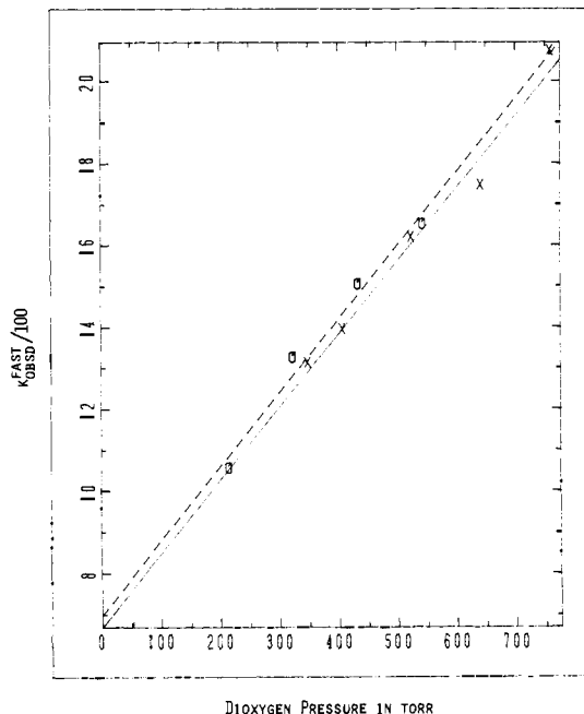
Figure 10. Plots of k_{\text{obsd}}^{\text{fast}} (after flash photolysis of DCIm-5-CO) vs. dioxygen partial pressure over toluene (0.45 M DCIm) at 20 \text{ }^\circ\text{C} : (O) [\text{CO}] = 1.09 \text{ mM}, 109 \text{ torr} , slope = 1.50 \times 10^5 \text{ M}^{-1} \text{ s}^{-1} ; (X) [\text{CO}] = 1.17 \text{ mM}, 117 \text{ torr} , slope = 1.48 \times 10^5 \text{ M}^{-1} \text{ s}^{-1} .
